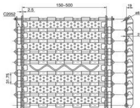
型号/Type: LJ:31.75mm (节距/pitch: 31.75mm)
