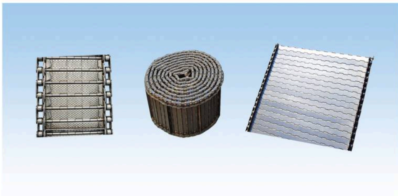
型号/Type: LJ:31.75mm (节距/pitch: 31.75mm)
