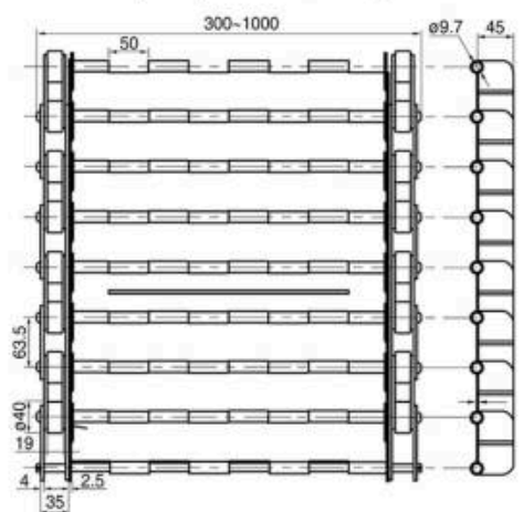
型号/Type: LJ:63.5mm (节距/pitch: 63.5mm)
