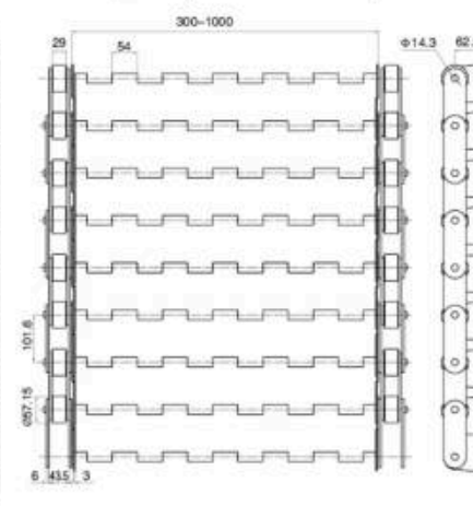
型号/Type: LJ:101.6mm (节距/pitch: 101.6mm)
